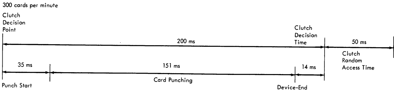
Figure 7. Card-Punch Timings (2540)
