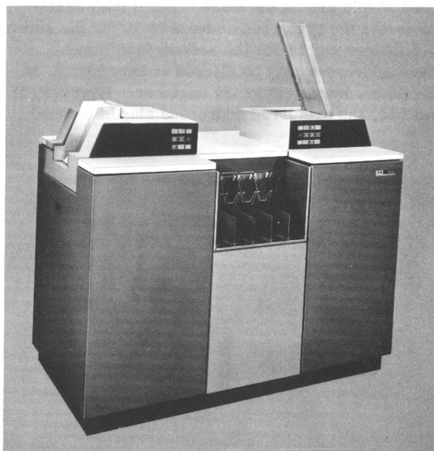
Figure 5. IBM 2540 Card Read-Punch
