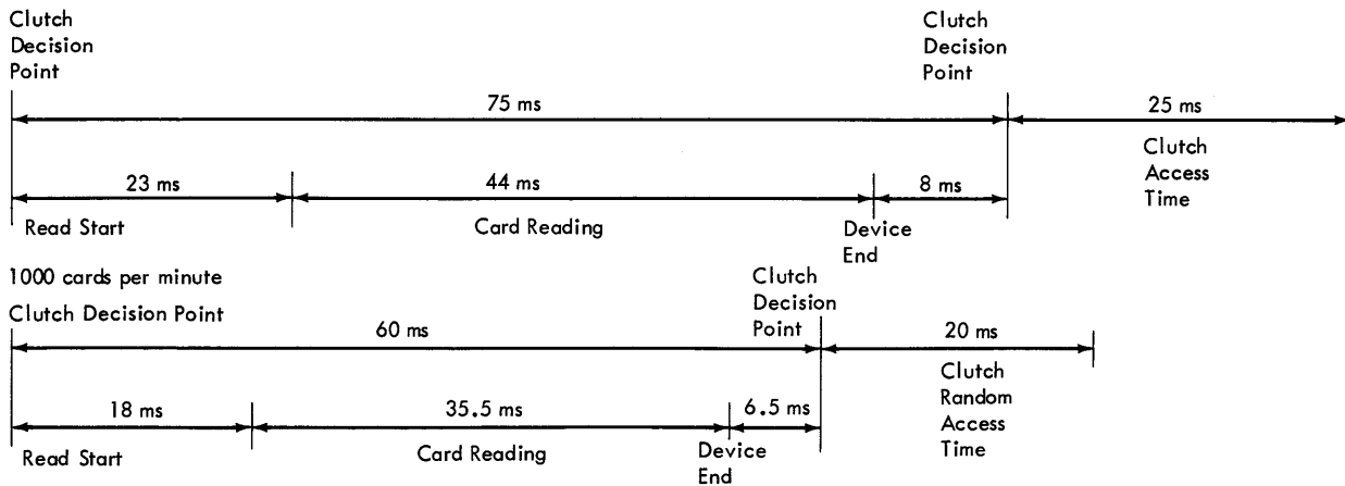
Figure 6. Card-Read Timings (2540)
